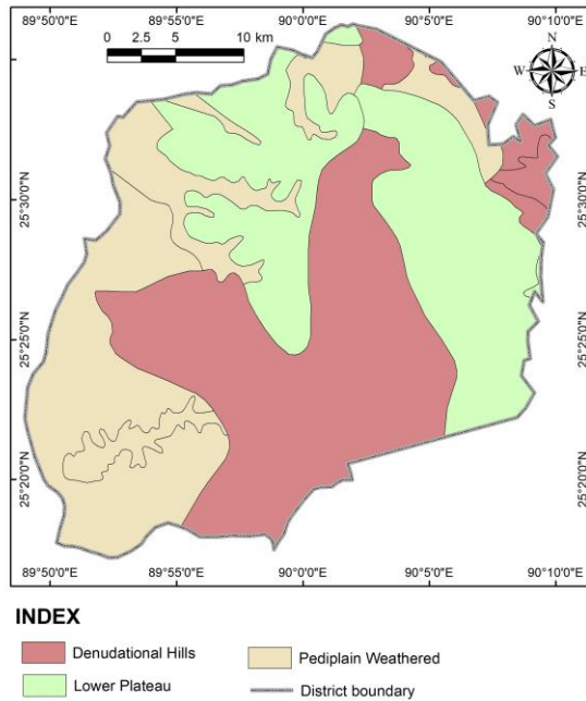
Fig. 1.5 GEOMORPHOLOGICAL MAP SOUTH WEST GARO HILLS, MEGHALAYA
