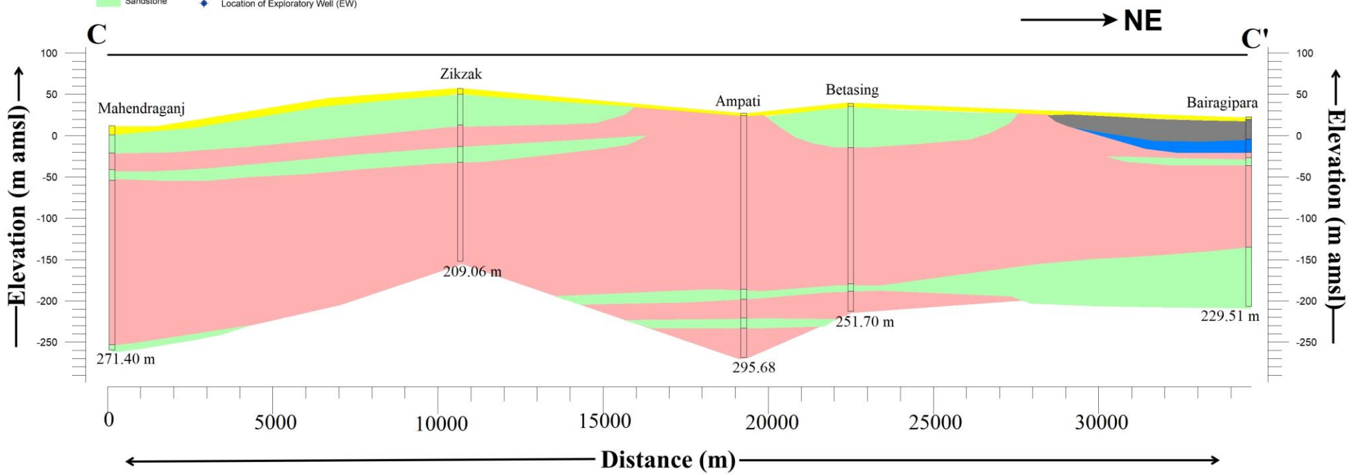
Fig 3.4 Hydrogeological cross section along C-C'
